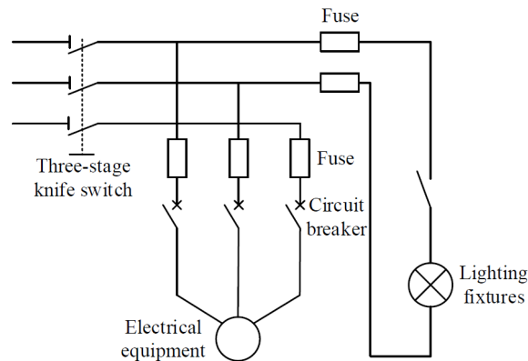
Figure 2: Construction chart of distribution line
