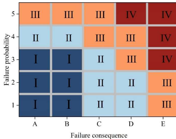
Figure 3: Risk matrix
