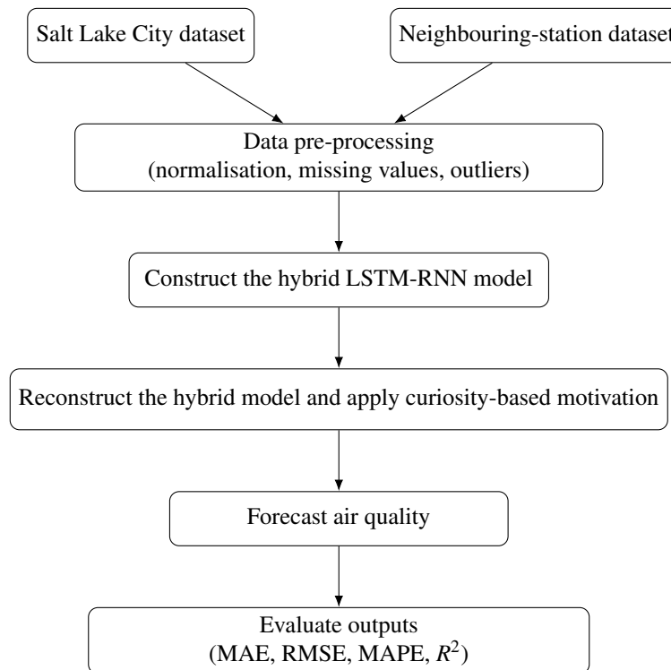
Figure 1: Cleaned reconstruction of the study workflow for smart-city air-quality forecasting.
