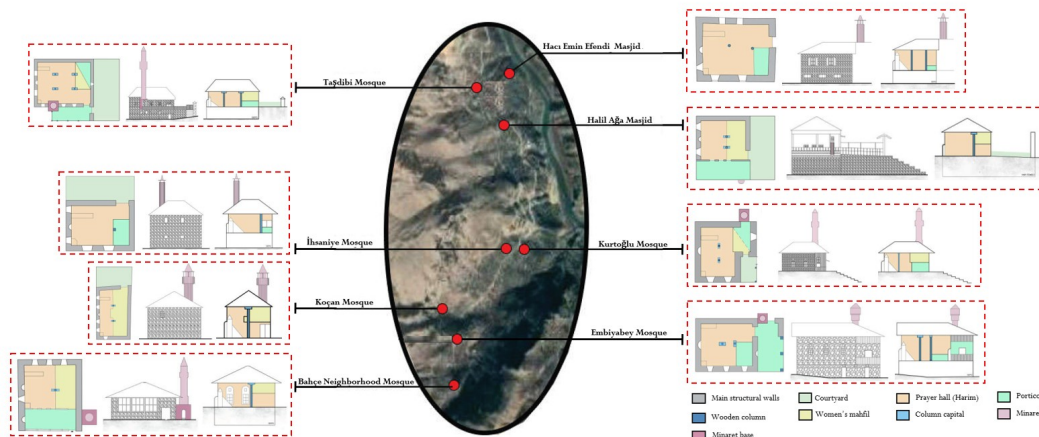
Figure 9. Measured drawings of the mosques located in the town center of Kemaliye, including plans, sections, and elevations (by the authors)
